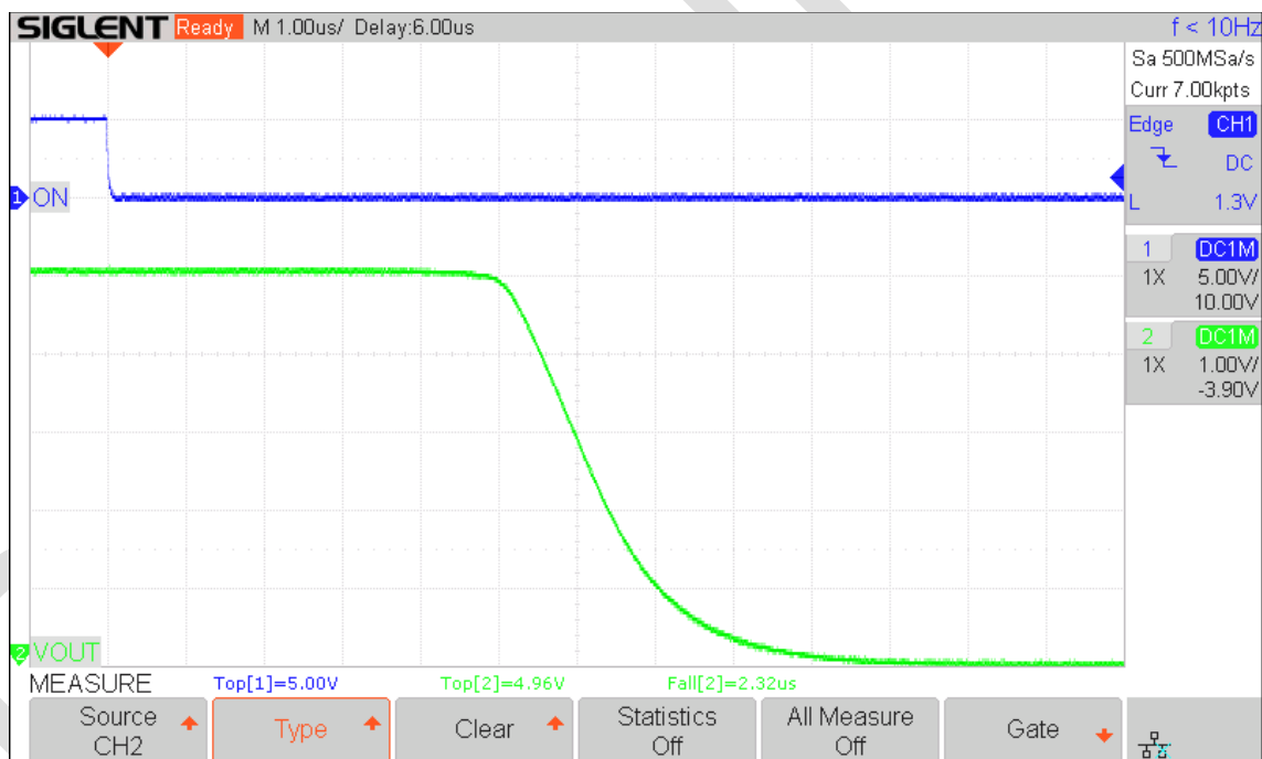
Figure 4. AM6U1101 typical power-down operation waveform. V_{IN} = 5V , C_{OUT} = 0.1\mu F , R_{LOAD} = 10\Omega
