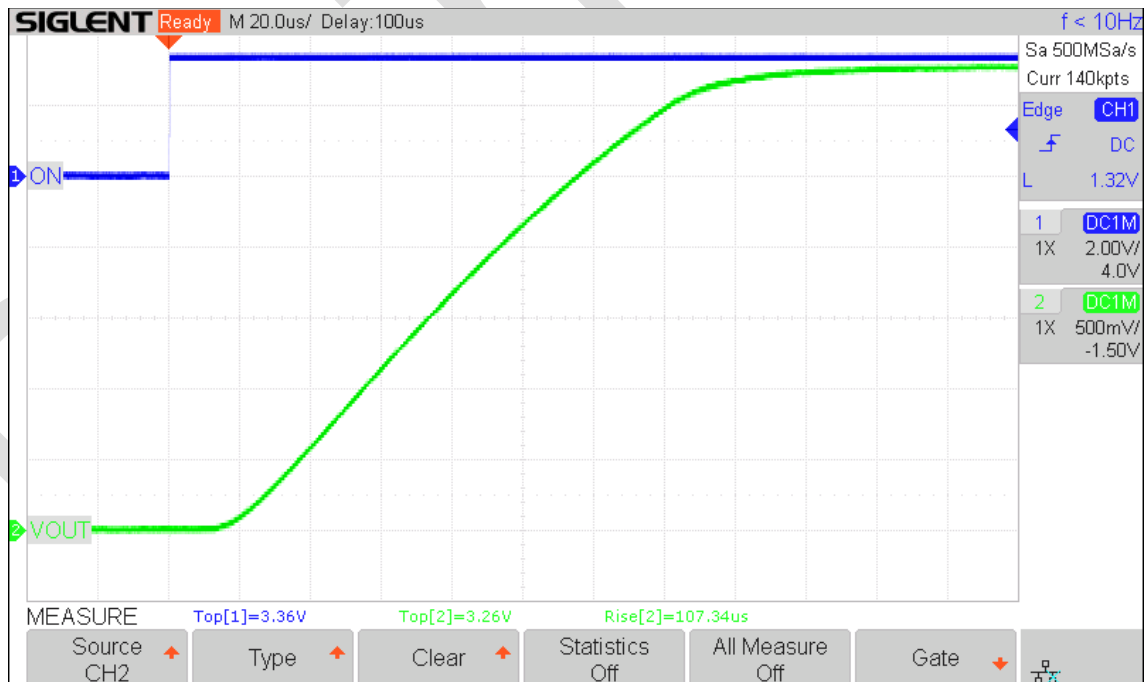
Figure 2. AM6U1101 typical power-up operation waveform. V_{IN} = 3.3\text{V} , C_{OUT} = 0.1\mu\text{F} , R_{LOAD} = 10\Omega
