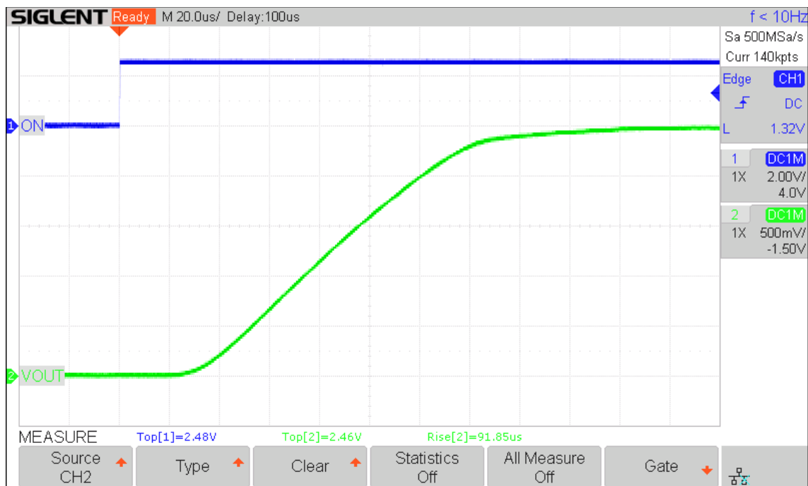
Figure 3. AM6U1101 typical power-up operation waveform. V_{IN} = 2.5V , C_{OUT} = 0.1\mu F , R_{LOAD} = 10\Omega
