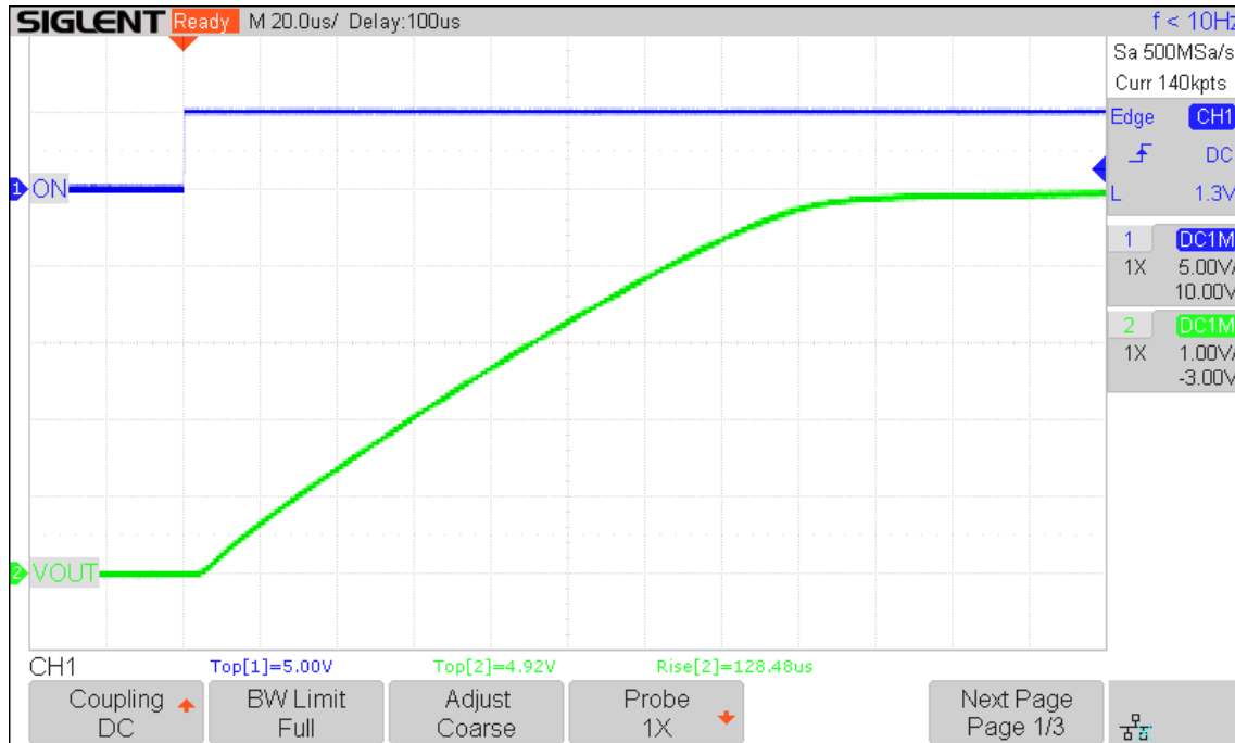
Figure 1. AM6U1101 typical power-up operation waveform. V_{IN} = 5\text{V} , C_{OUT} = 0.1\mu\text{F} , R_{LOAD} = 10\Omega
